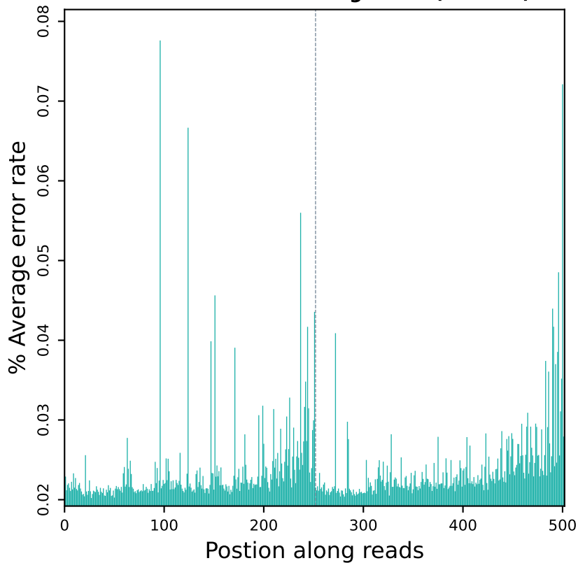
Error rate distribution along reads (R20116)
